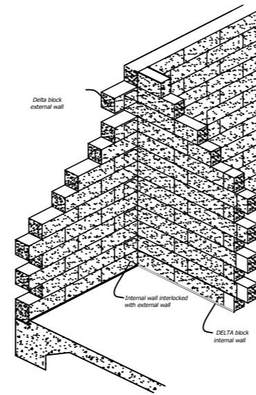
Intersection Between DELTA Block Walls N.T.S.
