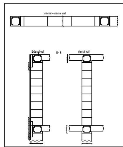
Typical Wall Section N.T.S.
