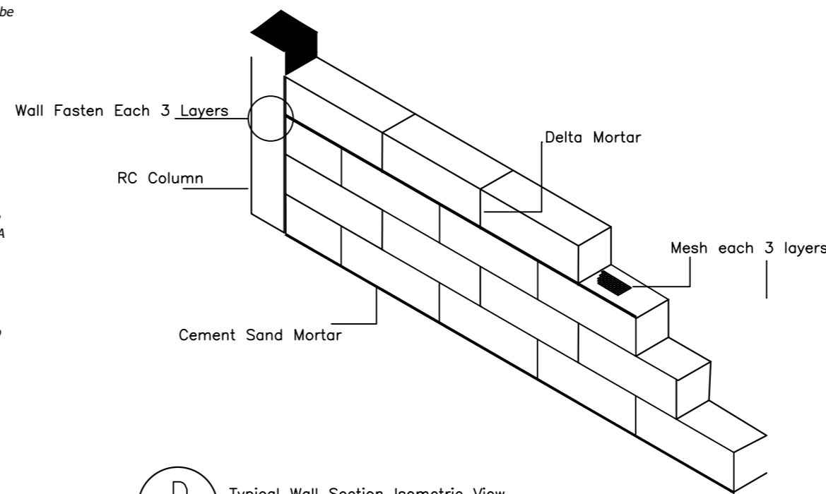
Typical Wall Section Isometric View N.T.S.
