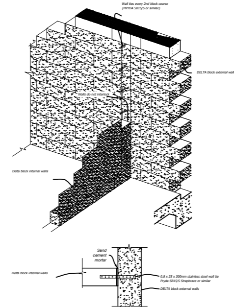
Alternative Internal to External Wall Intersection N.T.S.
